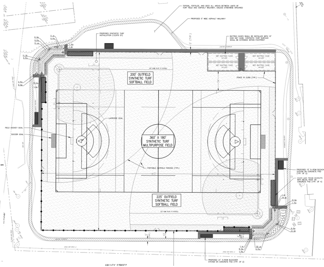
Ritzer: updated scope drawing showing substantially increased field/turf areas as well as event/sport features, fencing, batting cages, dugouts, etc. There is also increased draining and other infrastructure related to the expanded scope
