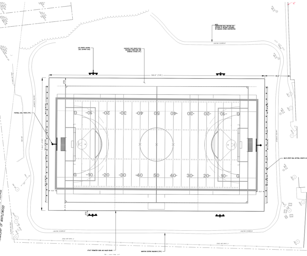
Ritzer: Original Scope drawing
