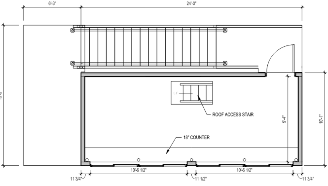
4 PRESSBOX SECOND FLOOR PLAN 1/4" = 1'-0"
