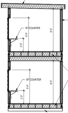
Press box "cut-through" view and elevation
