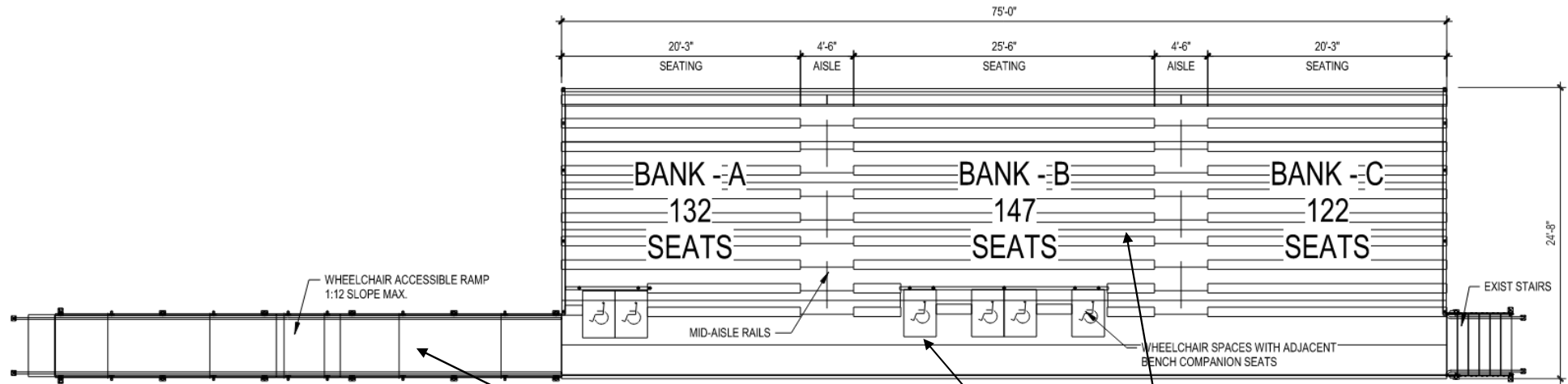
1 VISITOR'S SIDE GRANDSTAN PLAN 1/8" = 1'-0"
