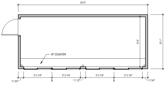
5 PRESSBOX FIRST FLOOR PLAN 1/4" = 1'-0"
